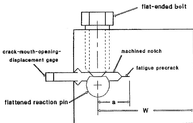
FIG. 3 Typical Test Arrangement for Constant Displacement K_{IEAC} Tests with Modified Bolt-Load Compact Specimen; H/W = 0.486
