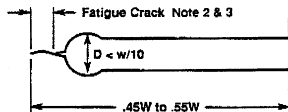
Slot Ending in Drilled Hole
