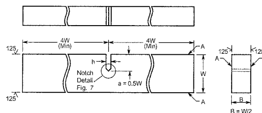
FIG. 4 Beam Specimen
