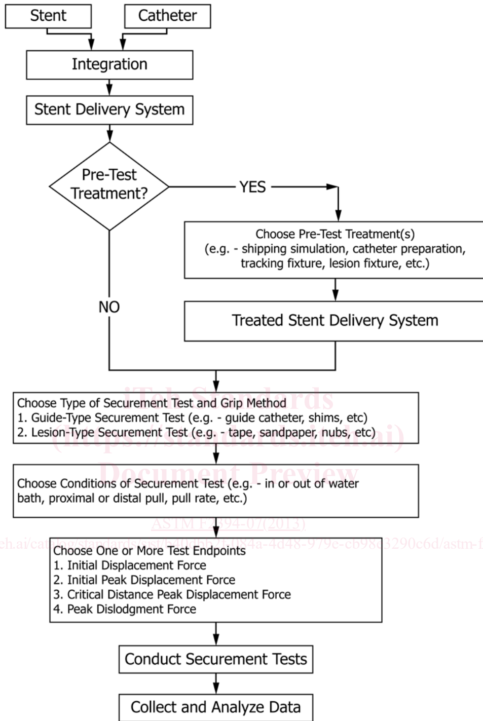
FIG. 1 Flowchart
