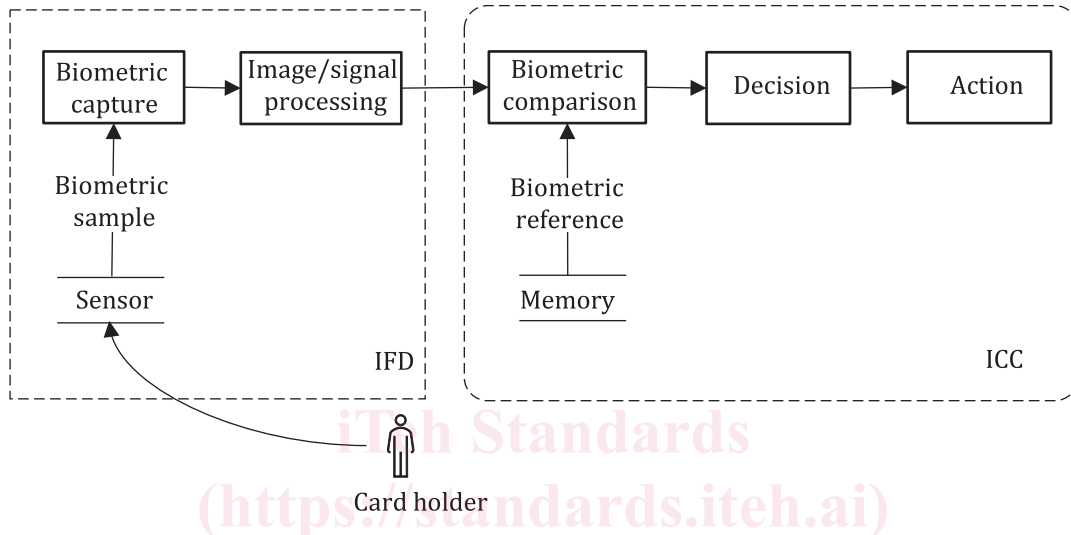
Figure 2 — General architecture of on-card biometric comparison (sensor-off-card)
