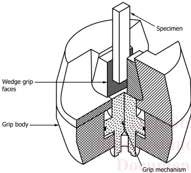
FIG. 3 Example of an Indirect Wedge-Type Grip Faces for a Face-Loaded Grip Interface
