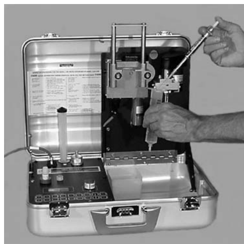
FIG. 5 Water Addition
