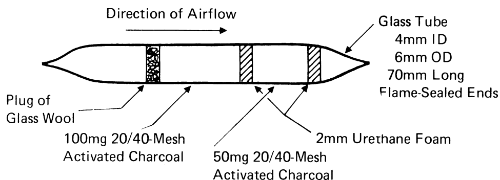
FIG. 1 Activated Charcoal Adsorption Sampling Tube
