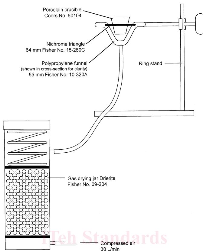
FIG. 1 Cooling Assembly
