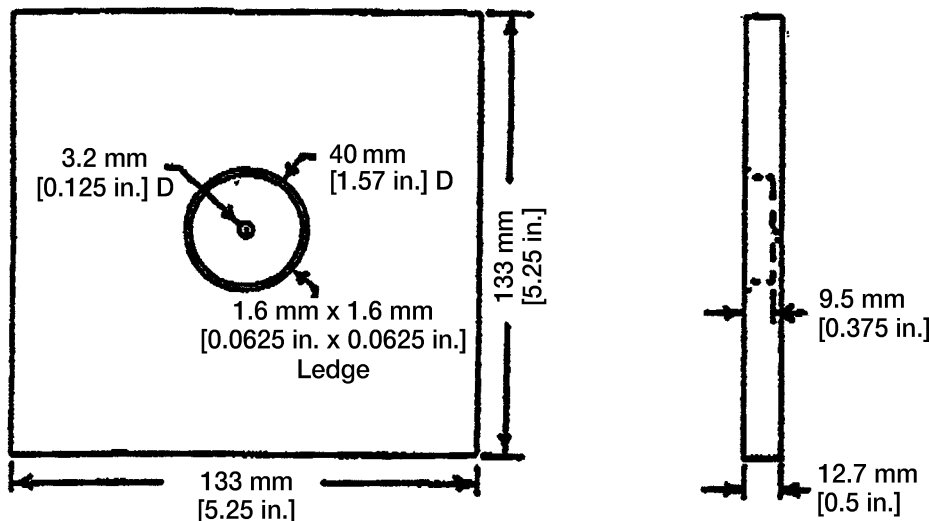
FIG. 2 Calorimeter Placement
