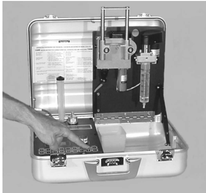
FIG. 8 Meter Adjustment
