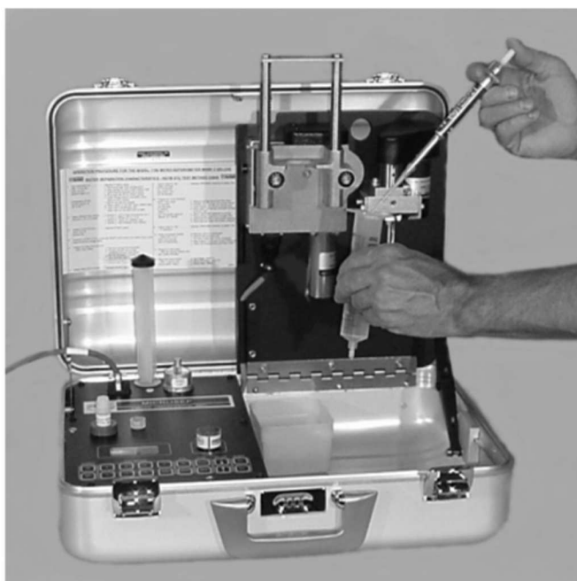
FIG. 6 Water Addition
