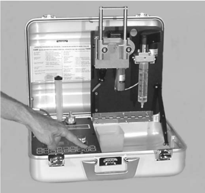
FIG. 8 Meter Adjustment
