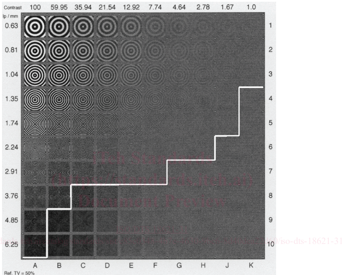
Figure 6 — Enclosed area above an index value threshold curve
