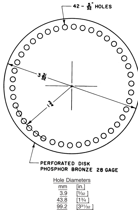
FIG. 56 Phosphor-Bronze Disk
