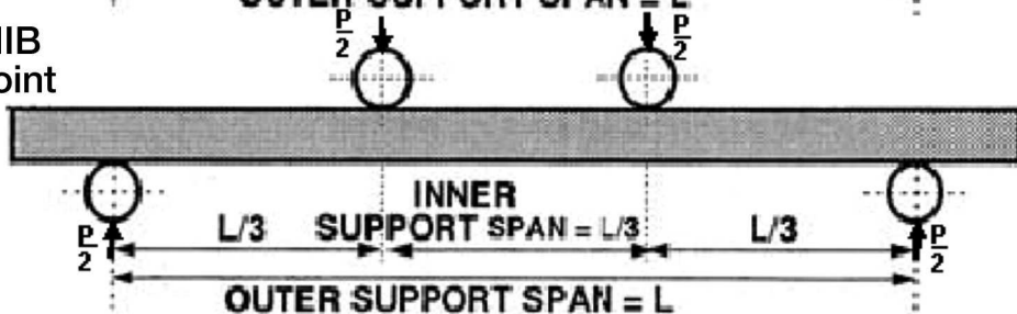
FIG. 1 Flexural Flexure Test Geometries and Force Diagram
