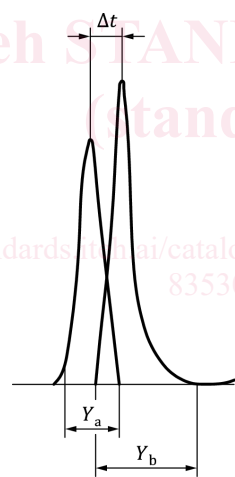
Figure 1 — Example of a chromatogram of a critical pair
