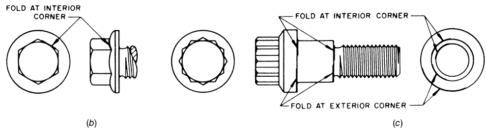
FIG. 5 Typical Folds
