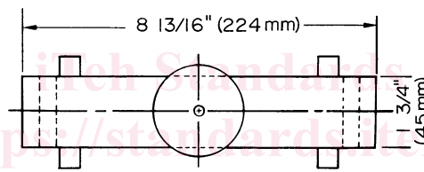
FIG. 1 Single-Shot Curved Electrode Details
