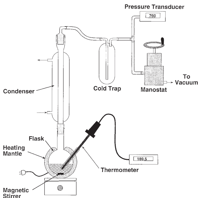
FIG. 2 Stirred-Flask Ebulliometer
