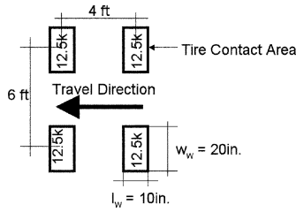
FIG. A1.2 Characteristics of Design Tandem
