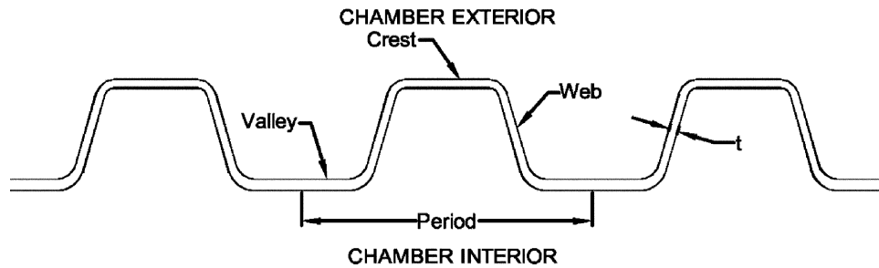
FIG. 2 Corrugation Terminology (Typical)
