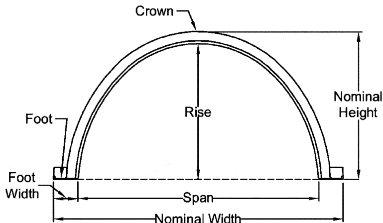
FIG. 1 Chamber Terminology (Typical)
