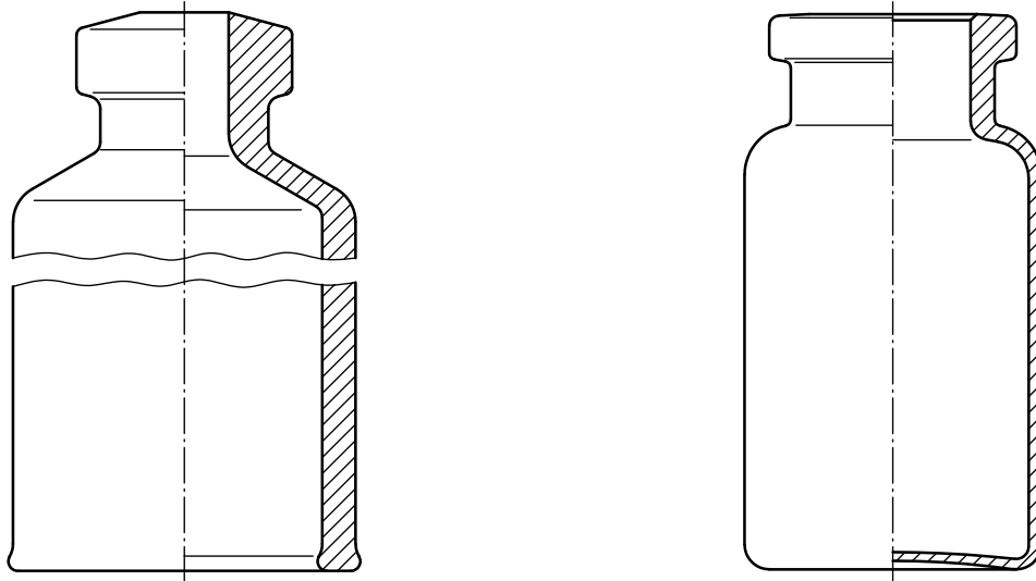
a) Example of a glass cylinder for a pen-injector / cartridge (see ISO 13926-1) b) Example of an injection vial made of glass tubing (see ISO 8362-1)
