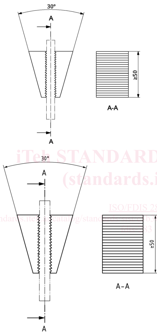
Figure 1 — Grip with transverse serrations
