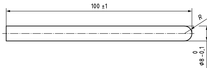
Figure 2 — 8 mm finger rod
