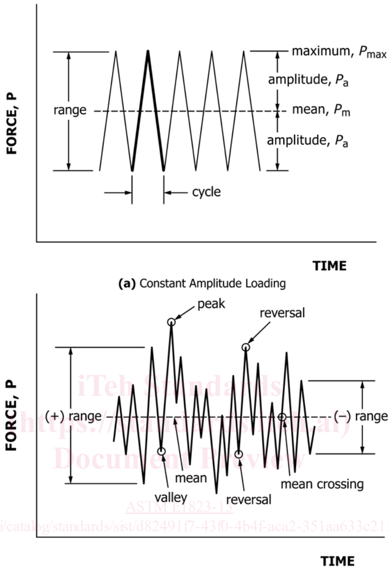
(a) Constant Amplitude Loading (b) Spectrum Loading FIG. 4 Fatigue Loading Basic Terms
