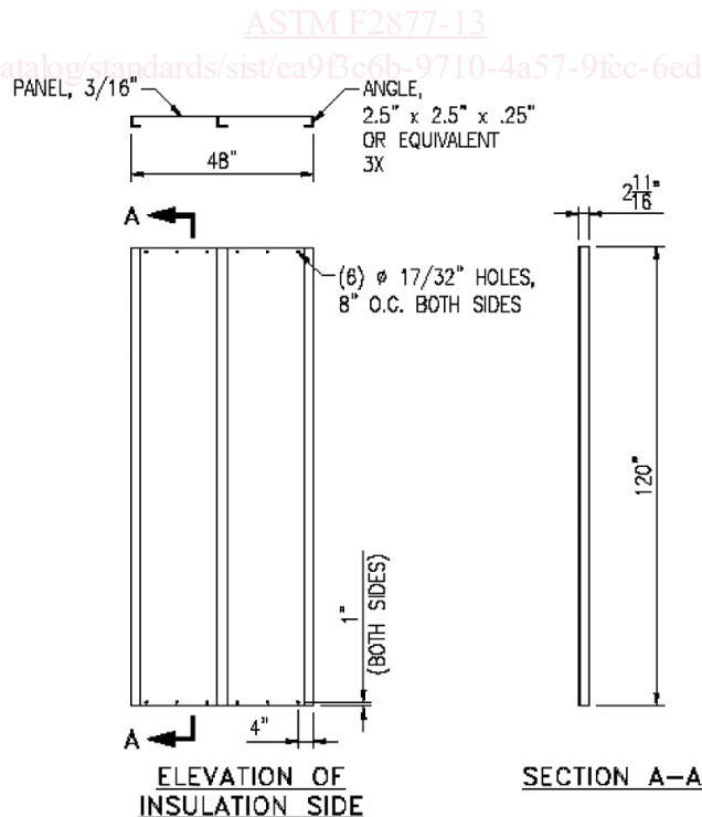
FIG. 1 Steel Test Specimen Construction Details for A-Class Bulkhead
