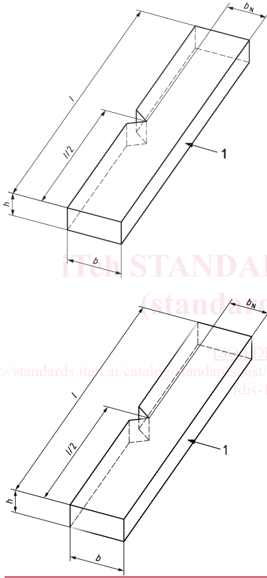
Figure 2 — Charpy edgewise impact (e) with single-notched specimen
