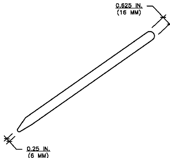
FIG. 1 Probing Tool
