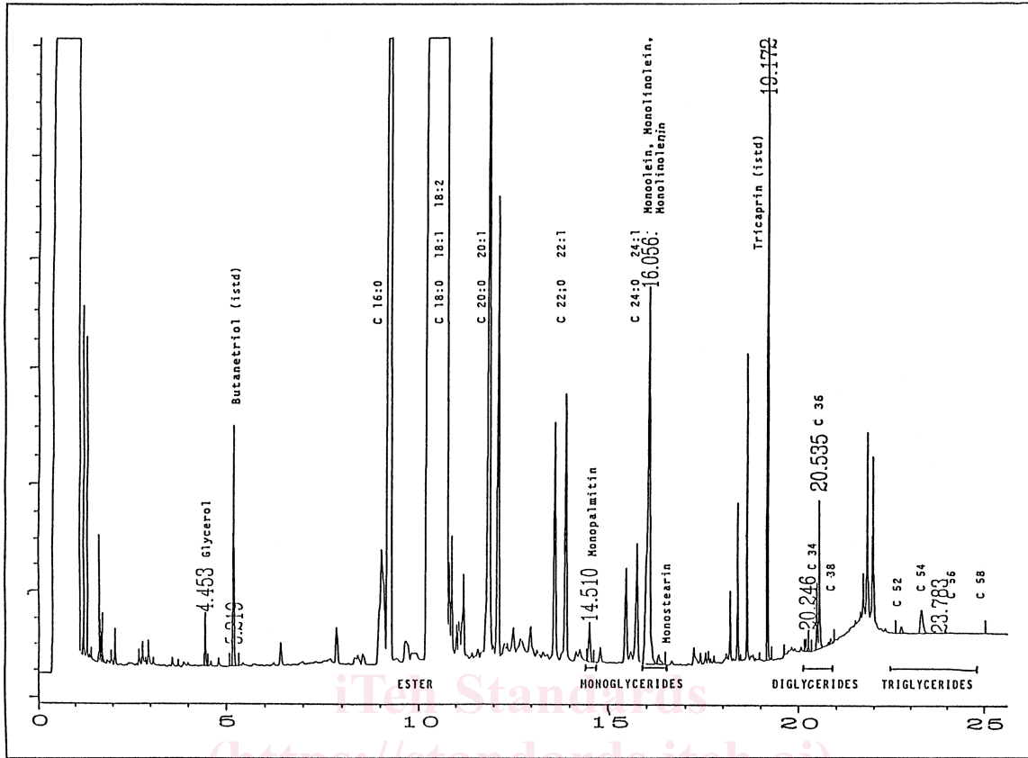
FIG. 1 Reference Chromatograms
