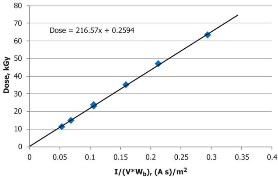
FIG. A1.1 Example of measurement of dose as function of average beam current I , conveying speed V and beam width W_b . Measured at an electron accelerator with beam energy 110 keV. K = 216.57 (kGy \cdot m^2) / (A \cdot s)
