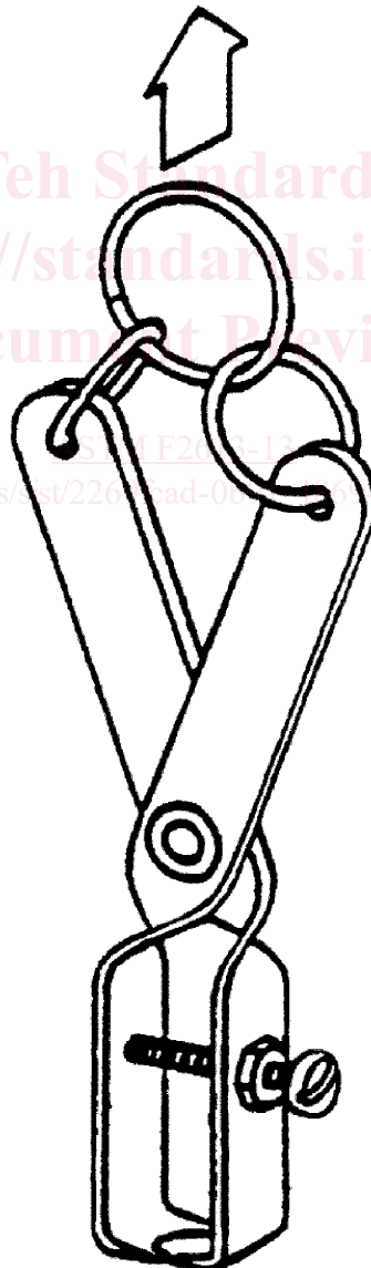
FIG. 1 Tension Test Adapter/Clamp
