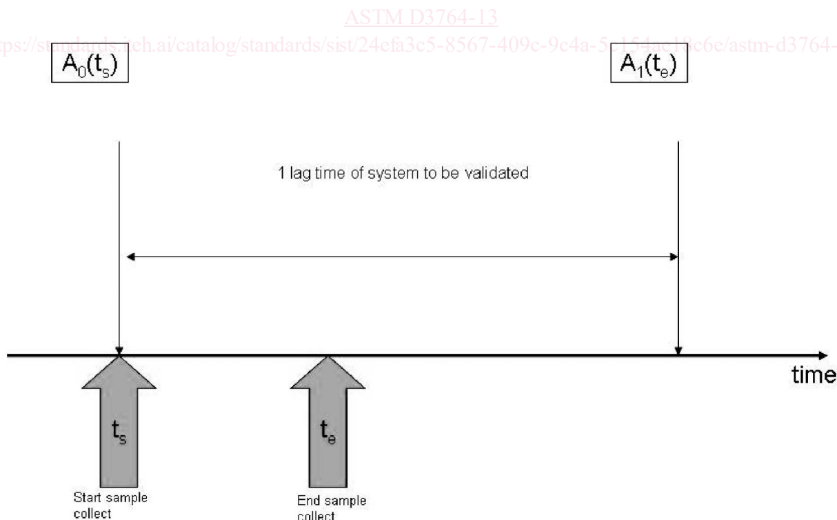
FIG. 3 Guidance for Recording Analyzer Result During Line Sampling (see 9.3.3.3)
