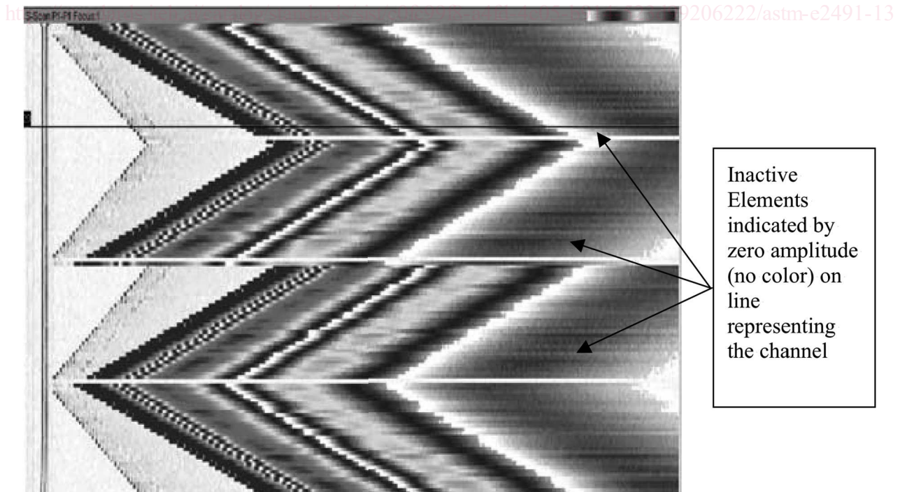
FIG. A3.1 Continuity Display for Phased-Array Instrument or Cable
