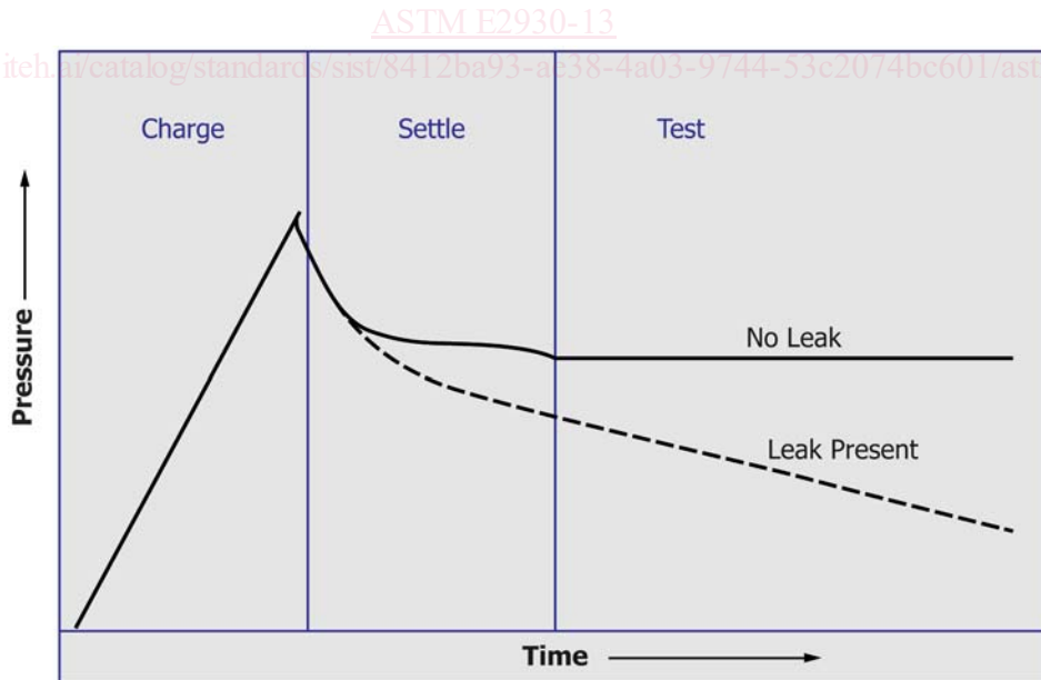
FIG. 2 Illustration of Pressure Decay Test Data
