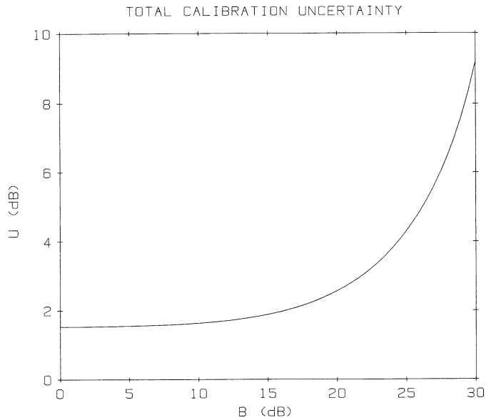
FIG. 28 Comparison—Estimated Uncertainty, U , of Primary, of the Calibration Frequency Response Data—Let M be the Largest Value of w_m over the Range 100 kHz to 1 MHz; Then, for any w_m , B = M - w_m , and Secondary Calibration Results, and the Uncertainty of for w_m Another SUT is \pm Having a Nominal Diameter of 0.5 in.
