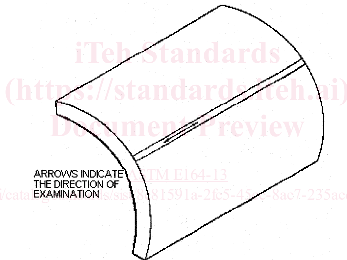
FIG. 15 Supplementary Technique 15, for Examining Longitudinal Welds, for Welds Ground Flush
