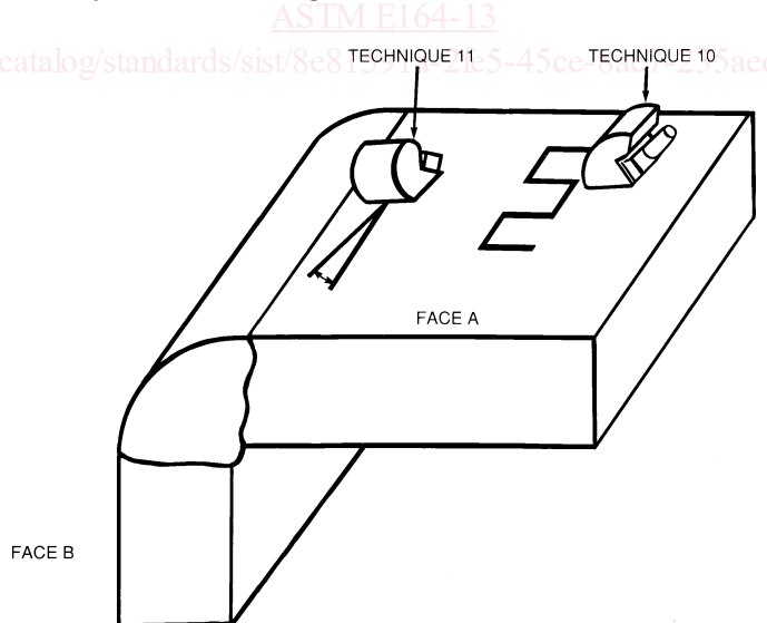
FIG. 11 Techniques 10 and 11, for Examining Full-Penetration Double-Fillet Corner Welds
