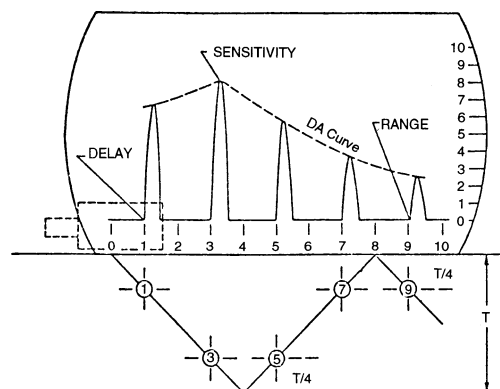
FIG. 1 Side-Drilled Hole
