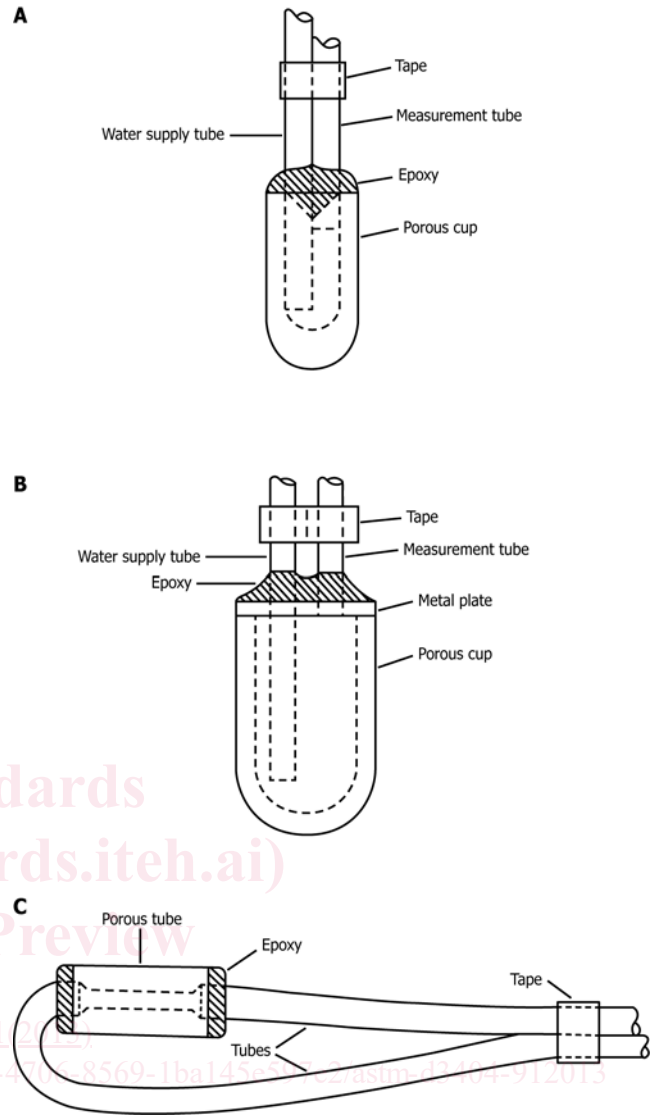
FIG. 3 Porous-Cup and Tube Designs
