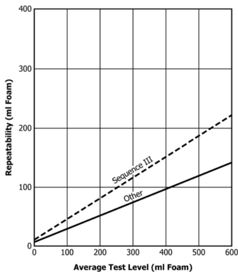
FIG. 3 Precision Chart—Repeatability
