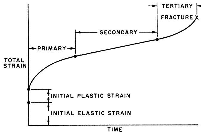
FIG. X2.1 Creep Curve
