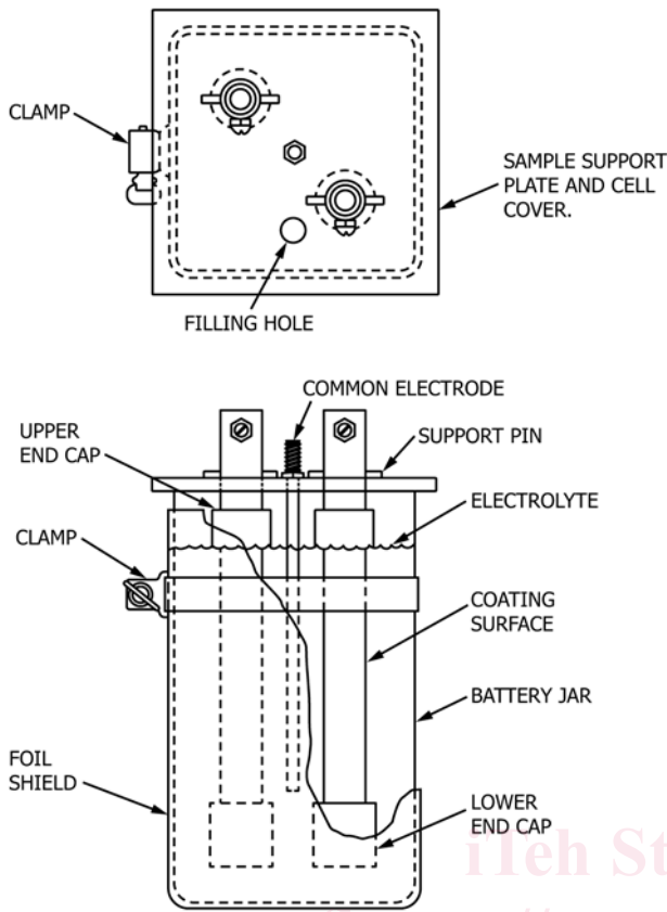
FIG. 1 Typical Test Cell
