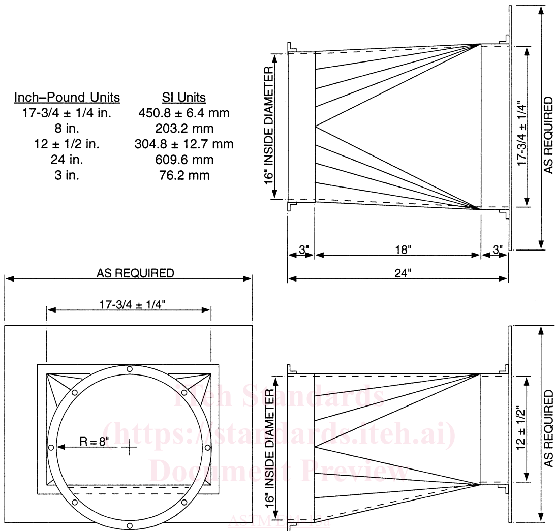
https://standards.iteh.ai/standards.iteh.ai/Document/Preview/ASTM-E84-13a-5b38b/astm-e84-13a FIG. 3 Typical Exhaust End Transition (Not a Construction Drawing)
