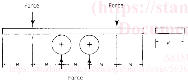
FIG. 11 Free Bend Support and Force
