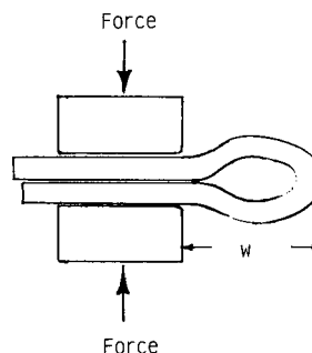
FIG. 13 Type 2 Flat-on-Itself Free Bend
