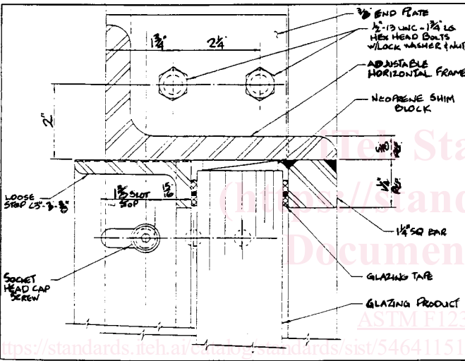
FIG. 3 Section of Glazing Material Test Frame
