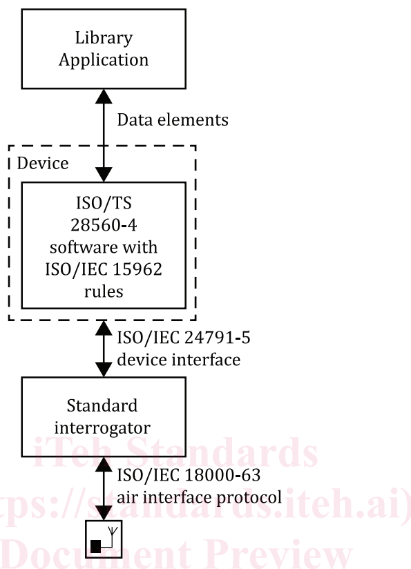
Figure 2 — Architecture with integrated data element software component
