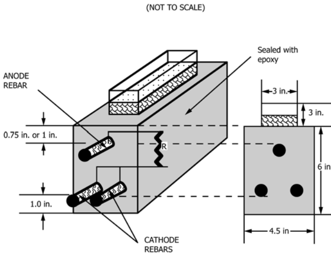
FIG. 1 Concrete Beam
