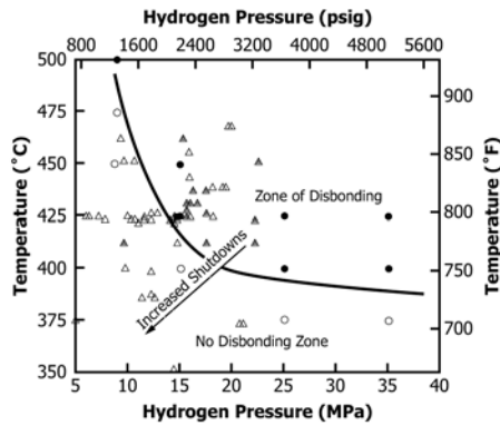
FIG. 1 Conditions of Hydrogen Partial Pressure and Temperature with Demonstrated Susceptibility to Hydrogen Disbonding in Refinery High-Pressure Hydrogen Service
