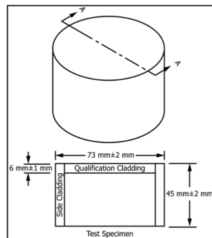
FIG. 3 Test Specimen Configuration
