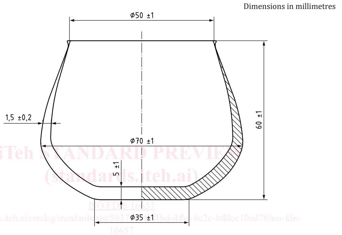
Figure A.1 — Dimensions of tasting glass for olive oil
