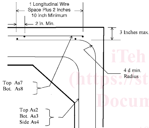
FIG. 6 Detail Option
