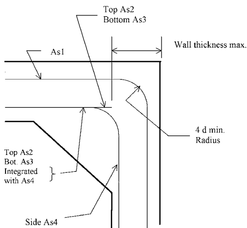
FIG. 7 Alternate Detail
