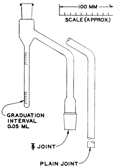
FIG. 2 Two-millilitre Receiver Showing Alternative Connections to Glass Still
