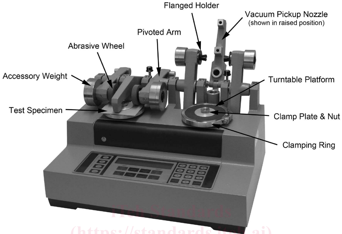
FIG. 1 Rotary Platform, Double-Head (RPDH) Platform Abraser
