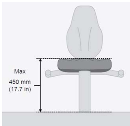
FIG. 5 Minimum Seat Dimensions – Height
