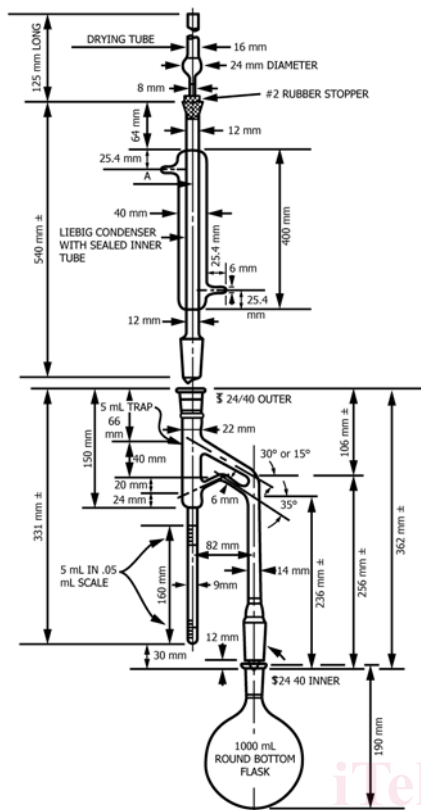
FIG. 1 Distillation Apparatus
