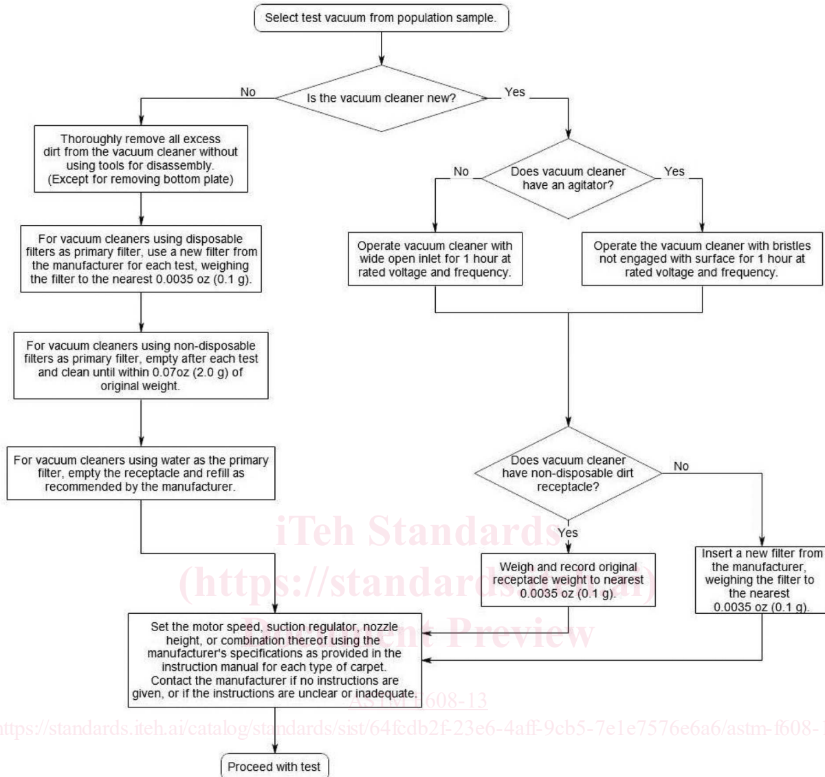
FIG. 2 Vacuum Cleaner Conditioning Procedure
